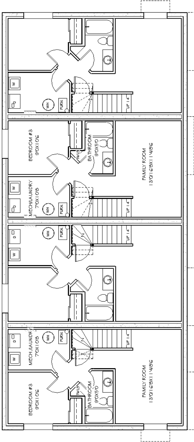
LOWER FLOOR LAYOUT OPTIONAL
