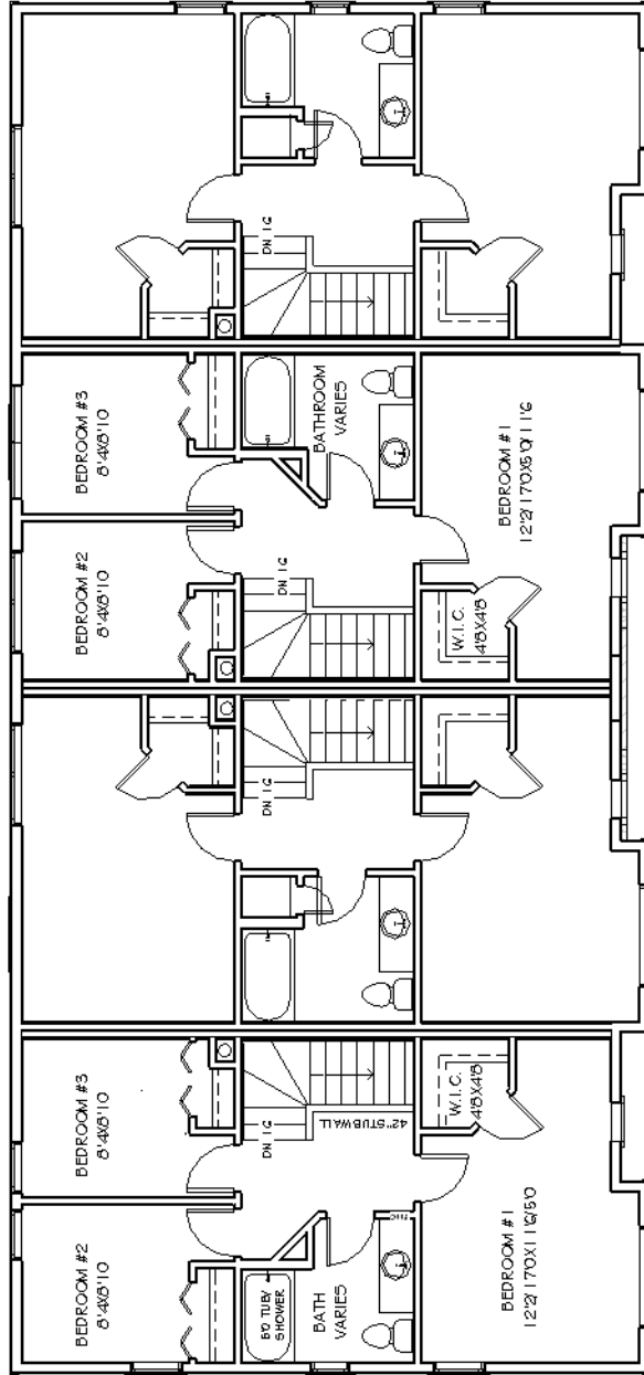
UPPER FLOOR PLAN 591 SQ. FT. 8'1" CEILING HT.
